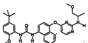
1-(5-tert-Butyl-2-methoxy-phenyl)-3-{4-[2-(2-methoxy-1-methylethylamino)-pyrimidin-4-yloxy]-naphthalen-1-yl}-urea;
